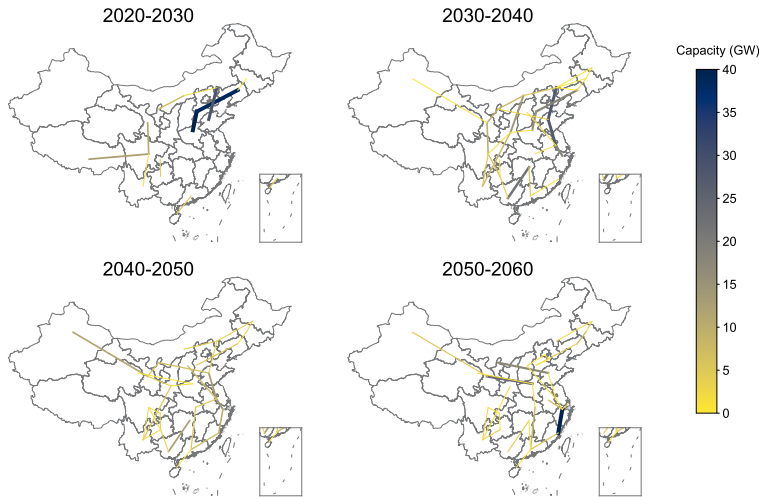
Fig. 5: Newly added inter-provincial transmission capacities under the 2°C Baseline scenario.
